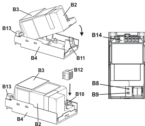
figure 7: mounting of an RL module
