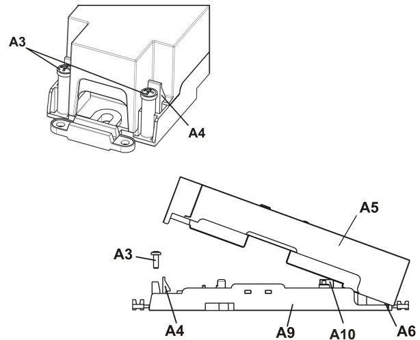
figure 3: Removing/Mounting the lid of the Control Module Box
