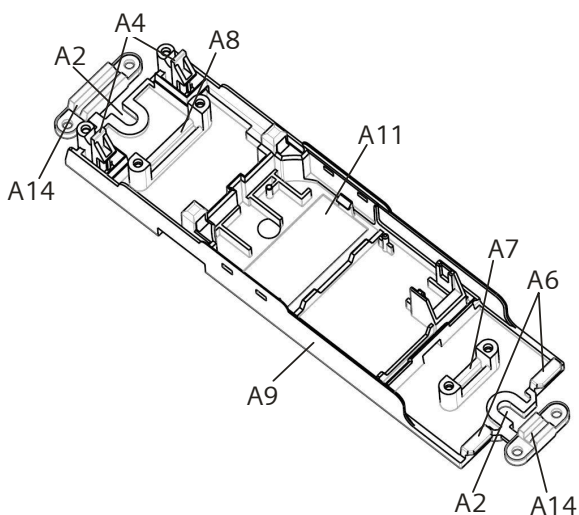
figure 2b: Mounting
