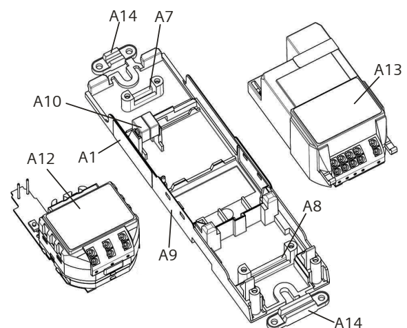
figure 4: mounting / dismounting of RS/RL modules
